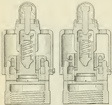
IMPROVED SAFETY VALVE.
